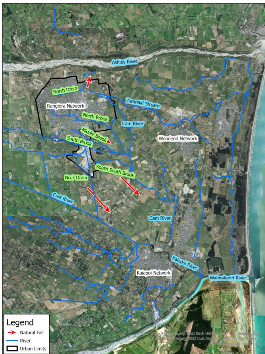
Figure 1: Rangiora network location plan
