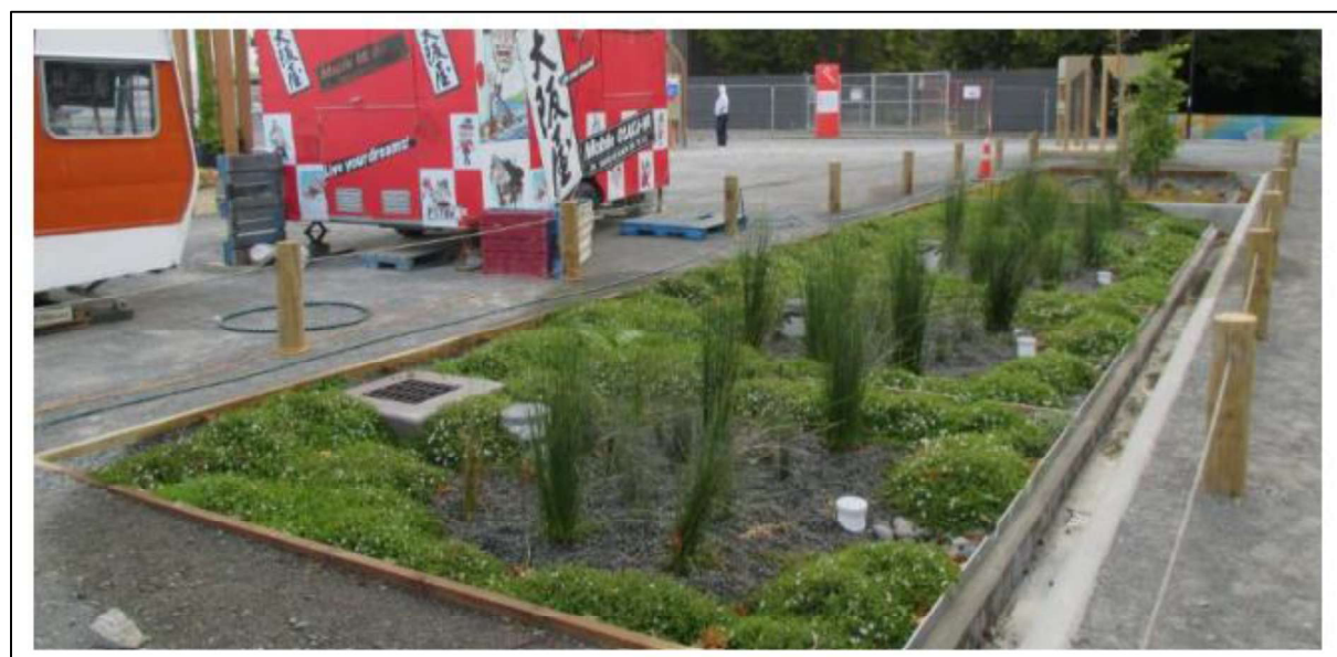
Figure 17: Example of a rain garden (Christchurch City Council, 2016)
