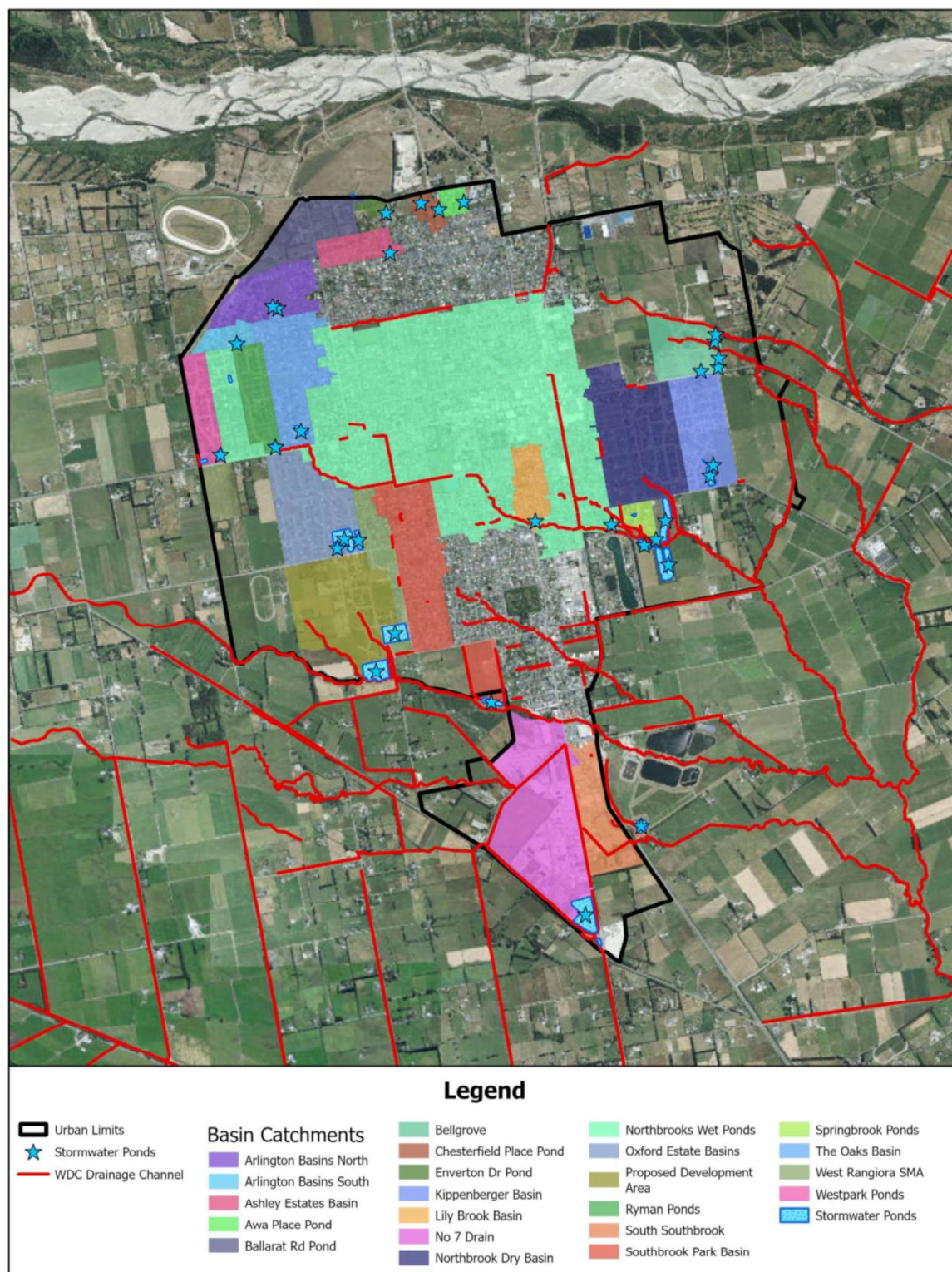
Figure 10: Stormwater Ponds within Rangiora
