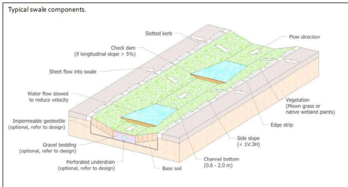
Figure 15: General components of a swale (Auckland Council, 2010)
