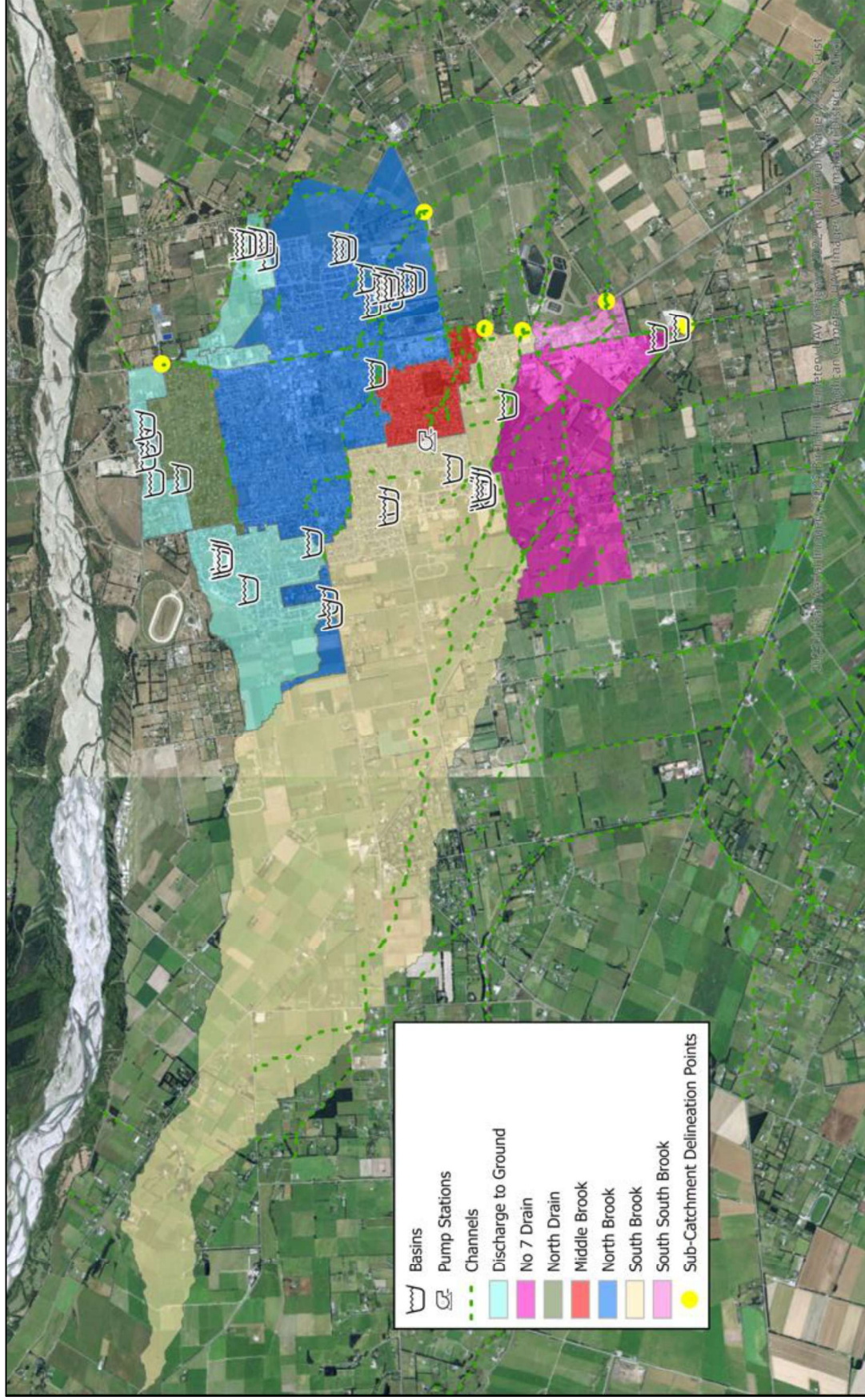
Figure 4: Rangiora stormwater drainage network and infrastructure
